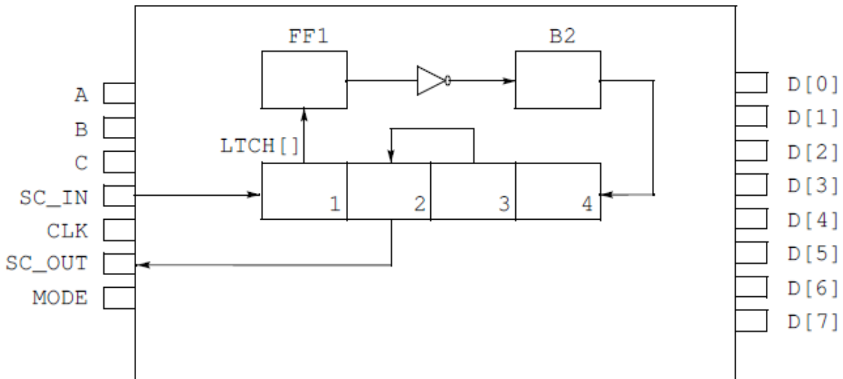
Figure 2-3 2: Example device with scan hardware
